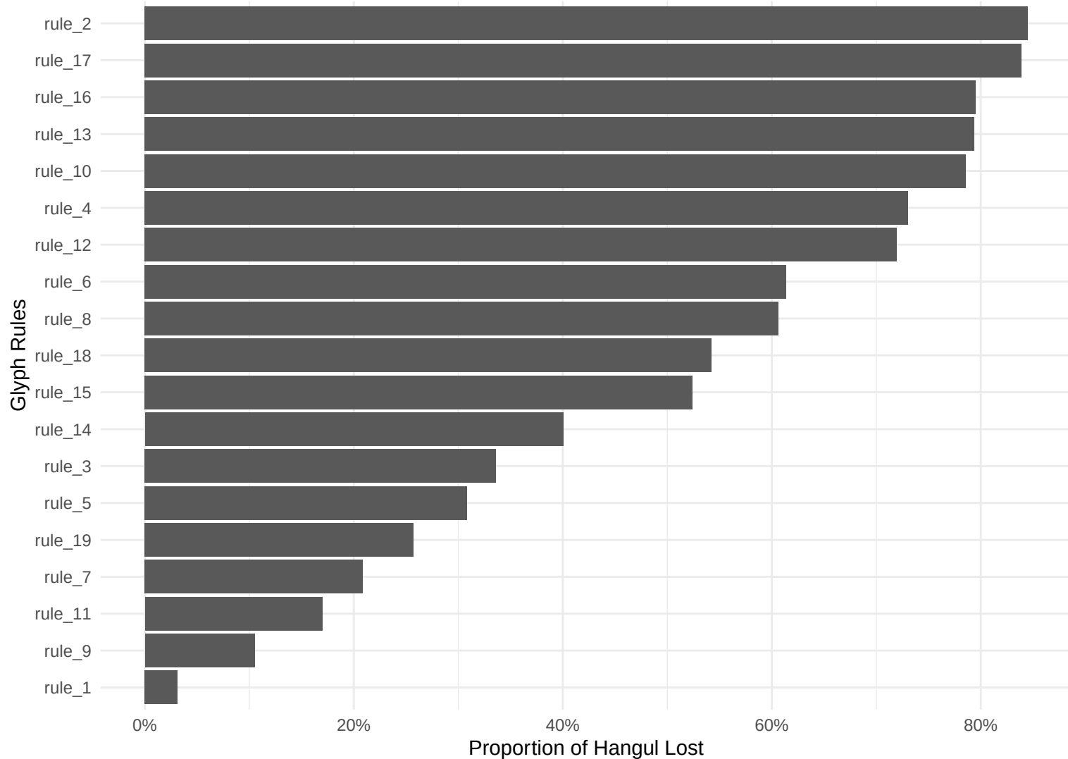
Effect of Rule Removal on Hangul (Weighted by Word Frequency)
